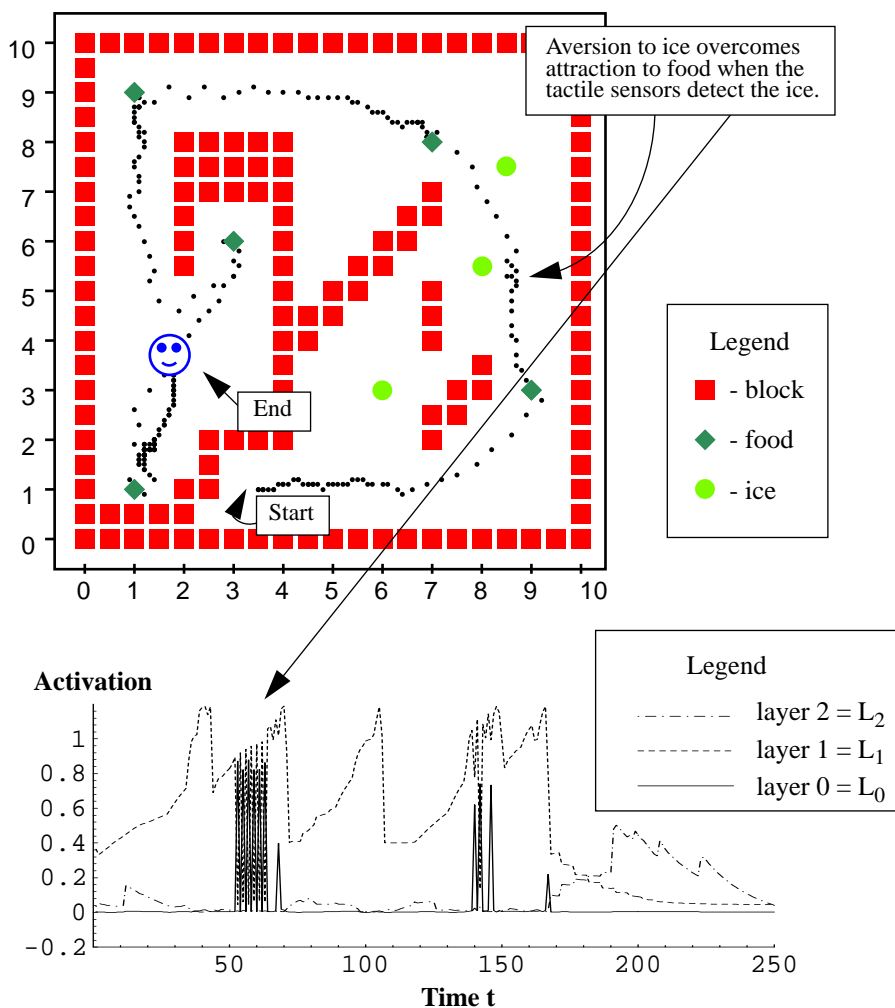
Figure 3: Addam's emergent behavior in a complex environment, with graph showing the activations of layers 0, 1, and 2.
