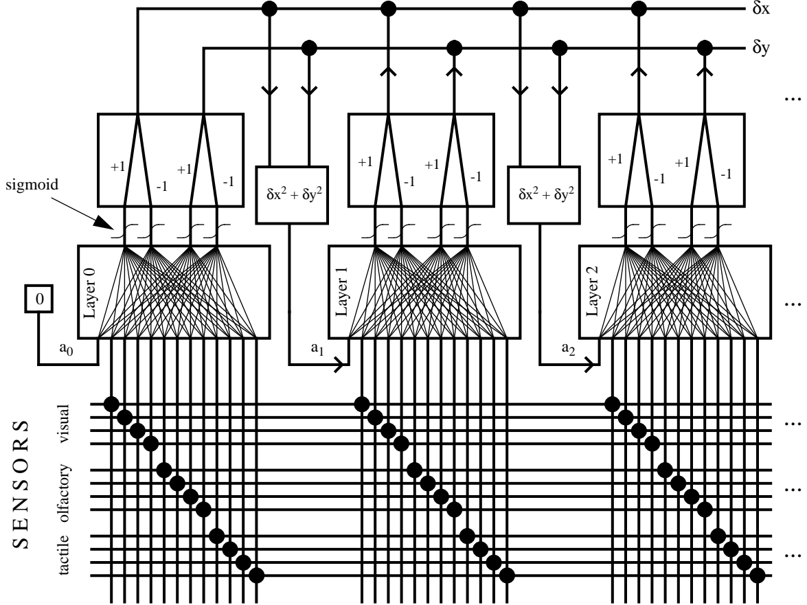
Figure 1: Addam's internal architecture.
